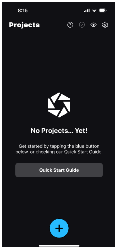
Obr. 10 knižnica Projects
